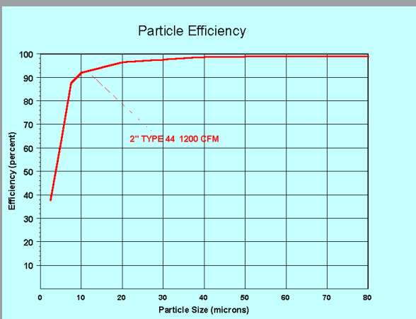
Particle capture efficiency at 1200 cfm.
